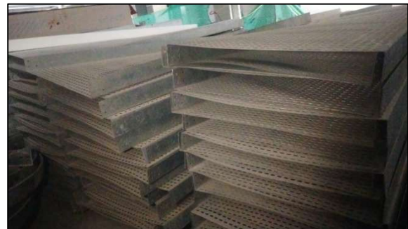
Description: 900*100mm GI Perf Tray Make: Electrofab Qty: 450 M Specification: 2mm, GI Perforated Tray
